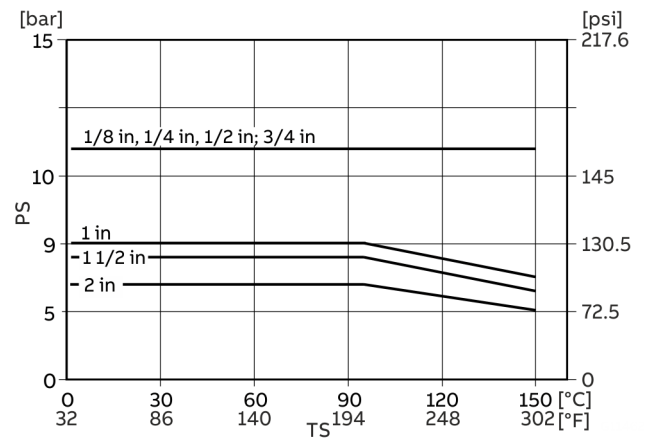
Figure 11: Material load curve for liquids
