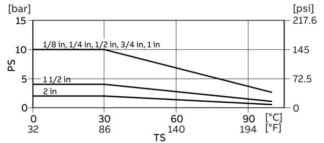
Figure 10: Material load curve for gas
