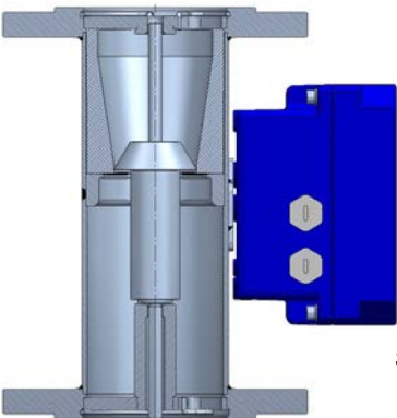
SM250 / AISI 316L with T-type float
